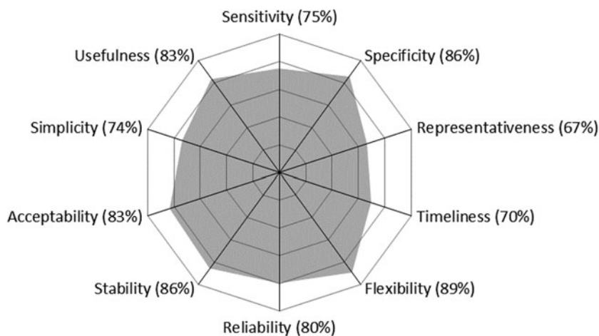
Fig. 3. Scores of RESAPATH obtained for the 10 OASIS attributes (indicated in proportions of the maximum possible score) in 2018.
